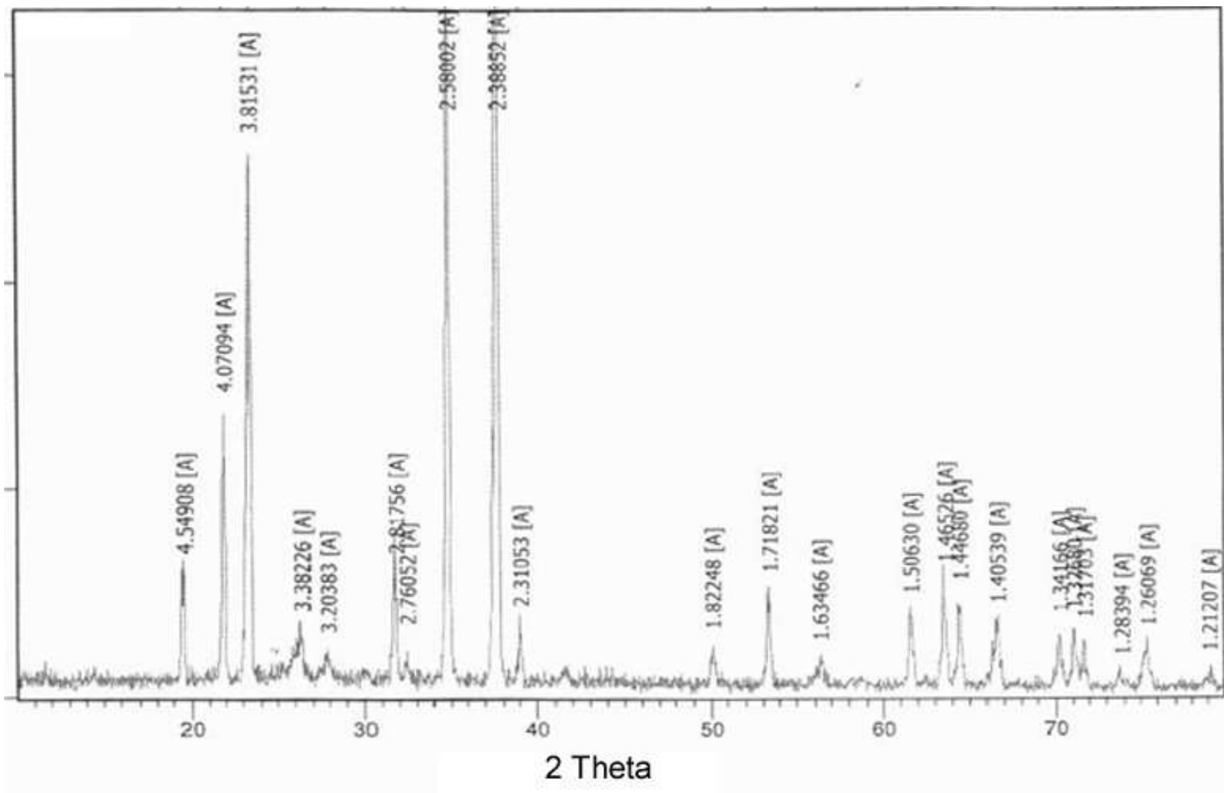
XRD pattern of B4C nanopowder, product 1540HK
